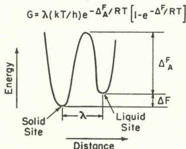
Fig. 4—Schematic Energy-Configuration Diagram at Solid-Liquid Interface.
