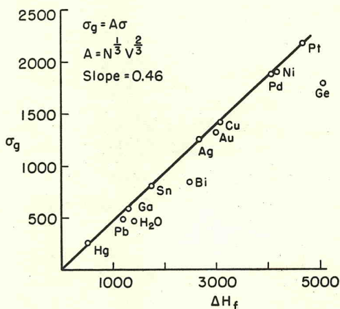
Fig. 2—Gram-Atomic Interfacial Energy as a Function of Gram-Atomic Heat of Fusion.
